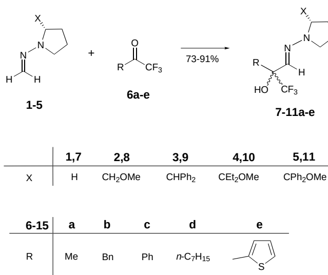
Scheme 1. Synthesis of \alpha -hydroxyhydrazones 7–11 .
