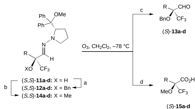
Scheme 2. Synthesis of compounds ( S,S )- 12 / S,S )- 14 and ( S )- 13 / S )- 15 . a) \text{BnBr} , \text{NaH} , \text{DMF} ; b) \text{MeI} , \text{NaH} , \text{THF} ; c) \text{Me}_2\text{S} ; d) \text{NaClO}_2 , t\text{BuOH} , isobutene.
