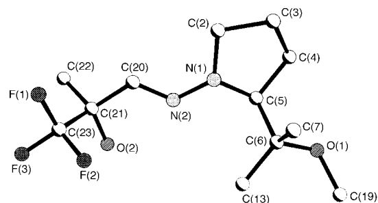
Figure 1. Crystal structure of ( R,S )- 11a . Phenyl groups have been omitted for clarity.
